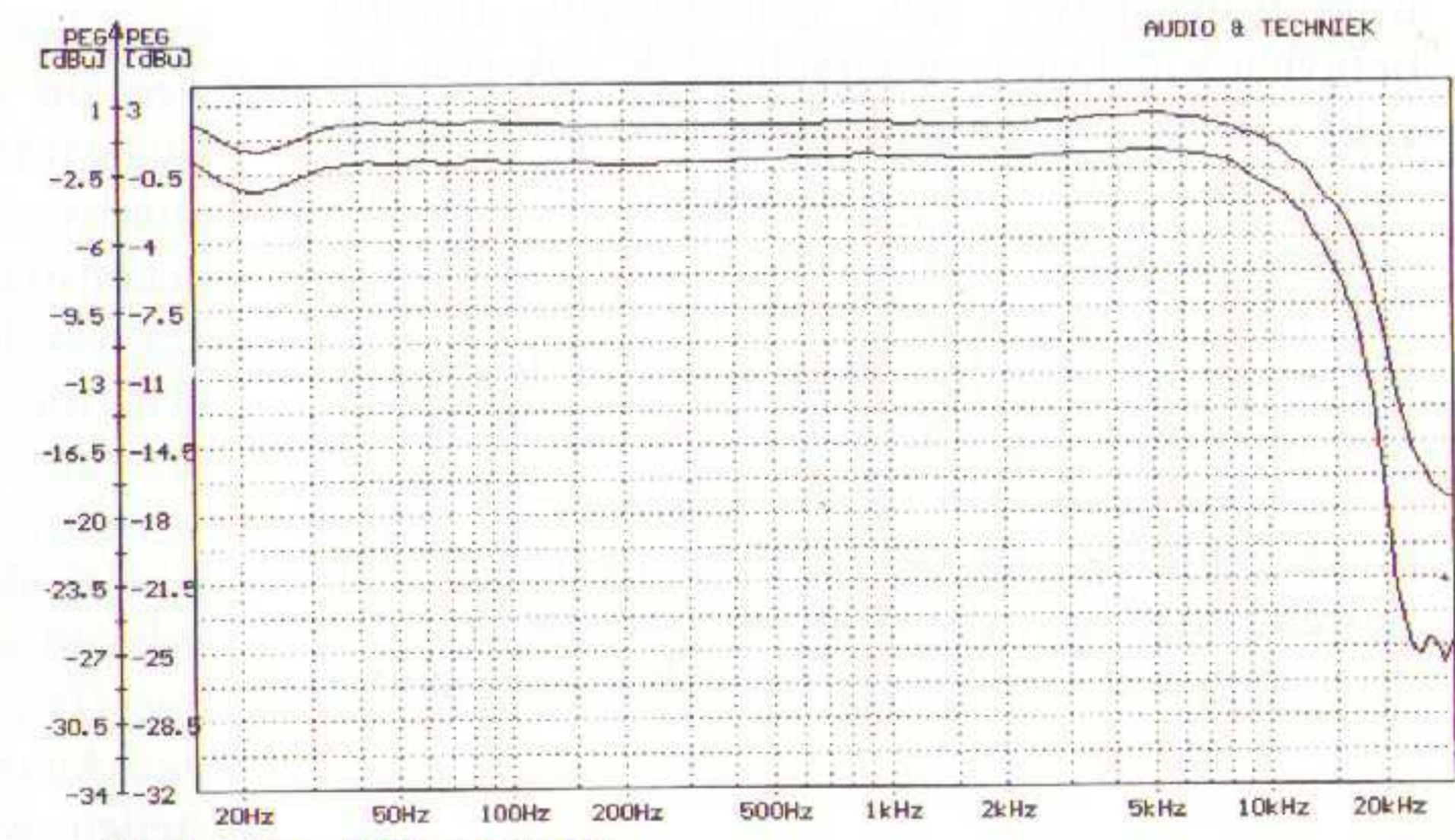
Technics RS-BX707
